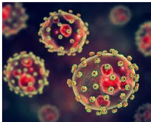
A picture of the haemorrhagic virus structure.
